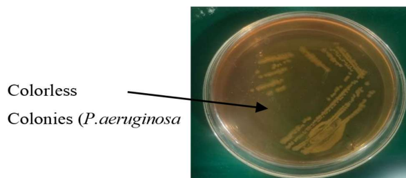
Fig 1: Colorless colonies on MacConkey agar.
