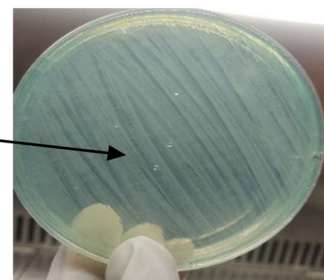
Fig 2: Results showing production of pyoverdine pigment on cetrimide agar.
