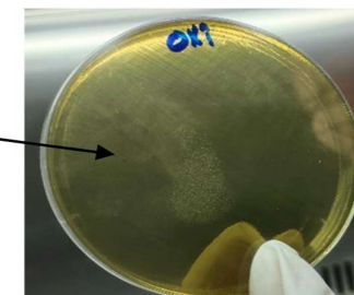
Fig 3: Results showing production of pyocyanin pigment on cetrimide agar.
